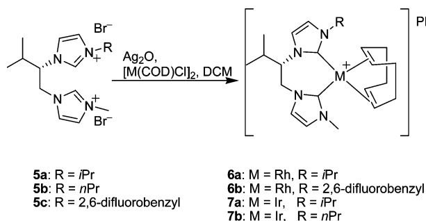
Scheme 3. Synthesis of complexes 6a,b and 7a,b . DCM = dichloromethane.
