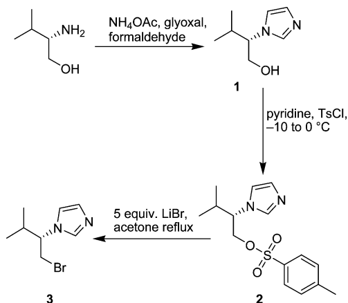
Scheme 1. Synthesis of the chiral imidazole bromide 3 .
