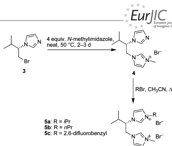
Scheme 2. Preparation of the bis(imidazolium) salts 5a–c .
