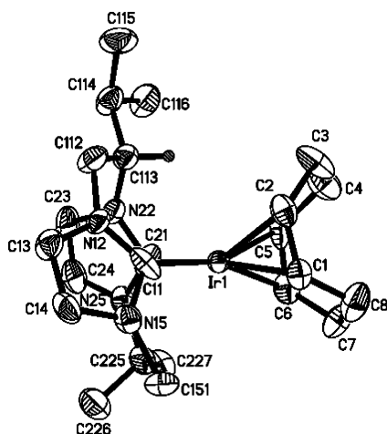
Figure 2. ORTEP diagram of 7a (thermal ellipsoids at the 50% probability level). Hydrogen atoms [except H at C(113)] and the counterion ( \text{PF}_6^- ) have been omitted for clarity. Selected bond lengths [Å] and angles [°]: Ir(1)–C(11) 2.068(4), Ir(1)–C(21) 2.015(6), Ir(1)–C(1) 2.204(3), Ir(1)–C(2) 2.147(4), Ir(1)–C(5) 2.186(5), Ir(1)–C(6) 2.197(4), Ir(1)–C(112) 3.552(14), Ir(1)–C(113) 3.112(13), Ir(1)–C(151) 3.442(7), Ir(1)–C(225) 3.628(8); C(11)–Ir(1)–C(21) 79.76(10), C(5)–Ir(1)–C(2) 80.95 (10), C(6)–Ir(1)–C(1) 81.19 (11).
