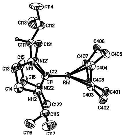
Figure 1. ORTEP diagram of 6a (thermal ellipsoids at the 50% probability level). Hydrogen atoms [except H at C(111)] and the counterion ( \text{PF}_6^- ) have been omitted for clarity. Selected bond lengths [Å] and angles [°]: Rh(1)–C(11) 2.035(3), Rh(1)–C(12) 2.026(8), Rh(1)–C(403) 2.204(5), Rh(1)–C(404) 2.218(4), Rh(1)–C(407) 2.173(3), Rh(1)–C(408) 2.202(6), Rh(1)–C(121) 3.174(14), Rh(1)–C(111) 3.561(16), Rh(1)–C(122) 3.620(6), Rh(1)–C(115) 3.448(7); C(11)–Rh(1)–C(12) 80.62(12), C(407)–Rh(1)–C(404) 81.17(11), C(408)–Rh(1)–C(403) 81.20(11).
